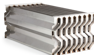
FLEXICHEVRON® STYLE VIII MIST ELIMINATOR.
