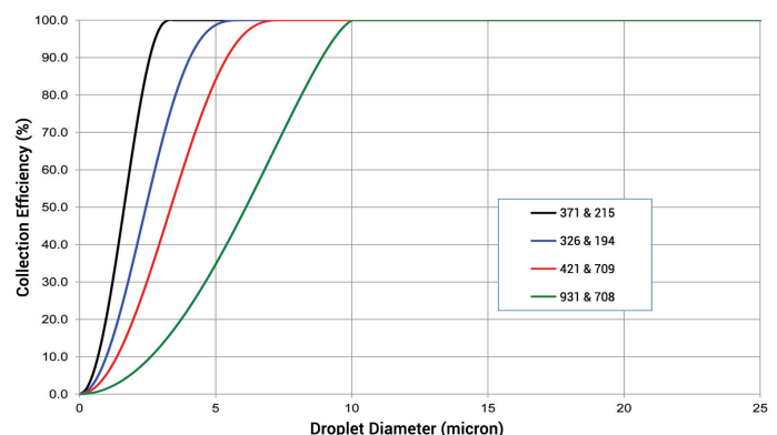
COMPARATIVE EFFICIENCIES OF VARIOUS DEMISTER® MIST ELIMINATOR STYLES IN AIR-WATER SYSTEM AT ATMOSPHERIC CONDITIONS.
